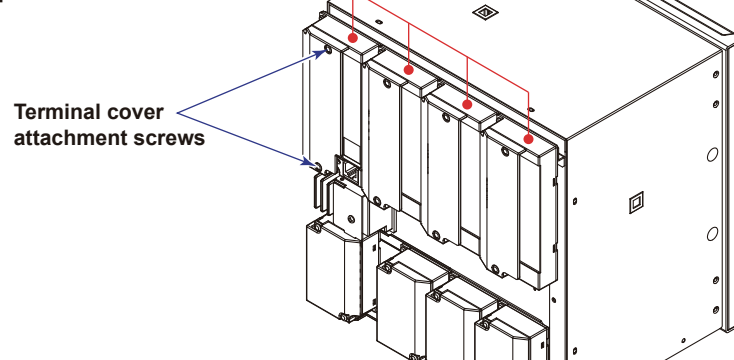
Optional terminal block
